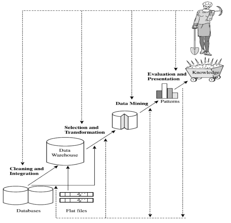
Architecture of KDD
